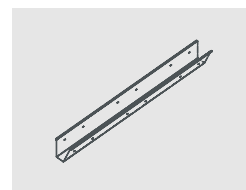
Calha Porta Cabos (p/Lineares) 1130 x 150 x 120 1330 x 150 x 120 1530 x 150 x 120
