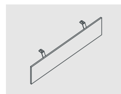
Painel Frontal (p/Lineares) 1050 x 18 x 290 1250 x 18 x 290 1450 x 18 x 290
